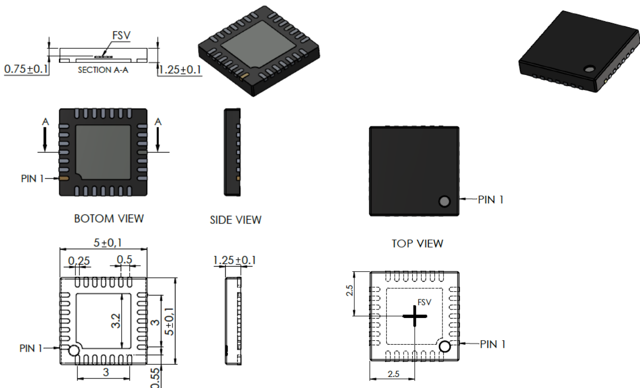
Figure 1: Dimensions of QFN 5x5 mm 2 package with 28 pins. The field sensitive volume (FSV) is located at the center of the package. Not to scale
