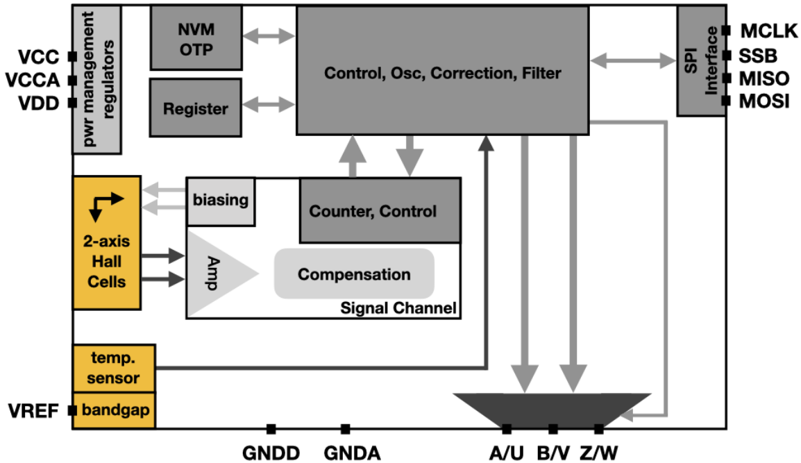
Figure 3: Block diagram of SENA2Dx
