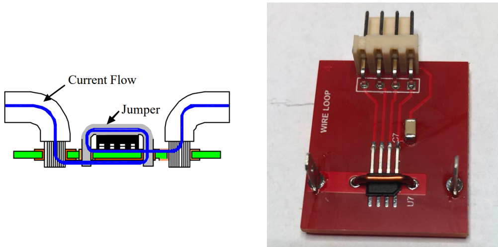
Figure 4: Left side: Current flow under and around sensor increase magnetic flux density in the chip Right side: Photo of EVBCS1Dx-SINGLE_WIRE_LOOP Evaluation Board – Top side
