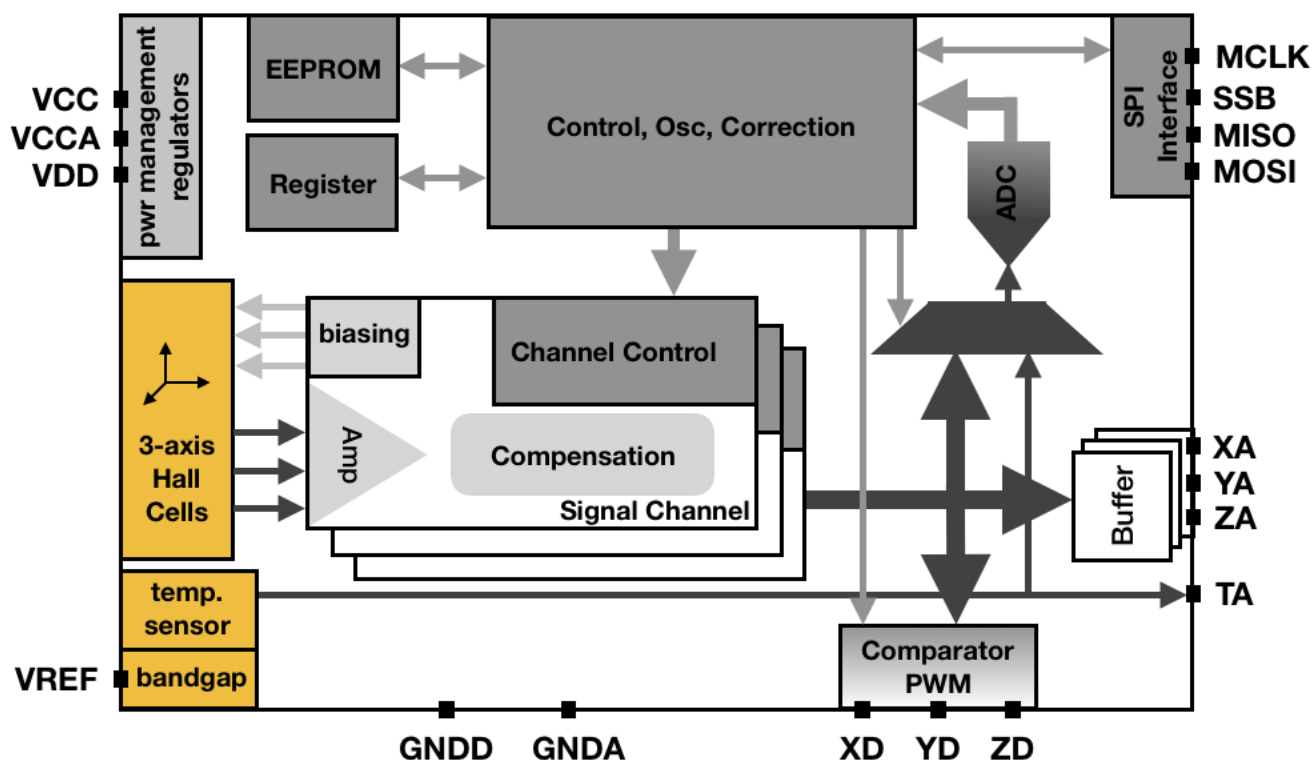
Figure 4: Block diagram of SENM3Dx
