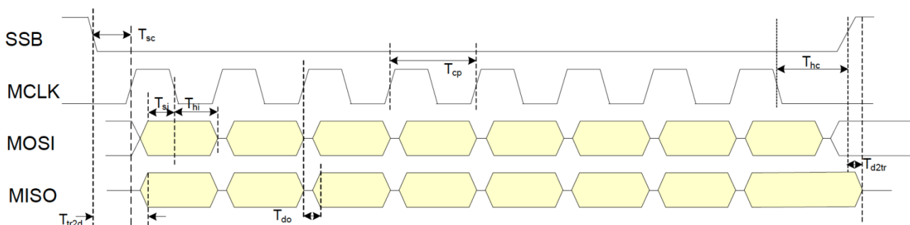
Figure 5: SPI Timing Parameter Definitions
