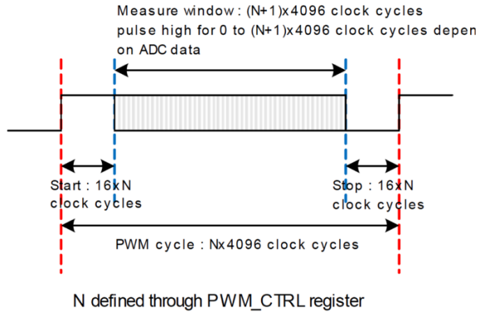
Figure 10: PWM Timing Diagram
