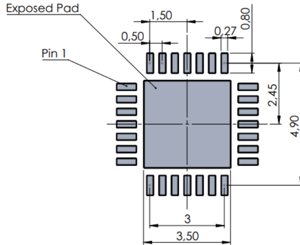
Figure 2: Recommended footprint. All dimensions are in units mm. If the center pin (exposed thermal pad) is used then it should be connected to GND.
