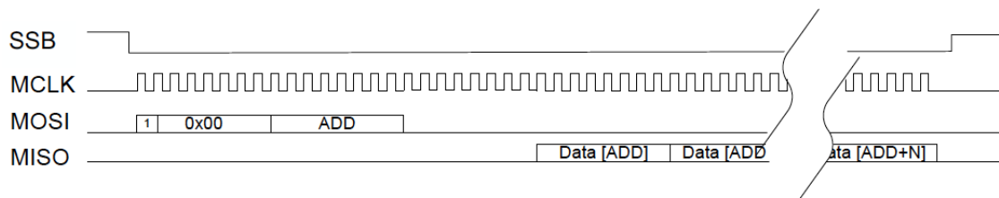
Figure 6: SPI Communication for Register Read Access Timing Diagram
