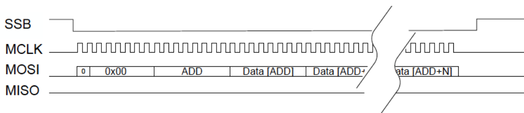
Figure 7: SPI Communication for Register Write Access Timing Diagram
