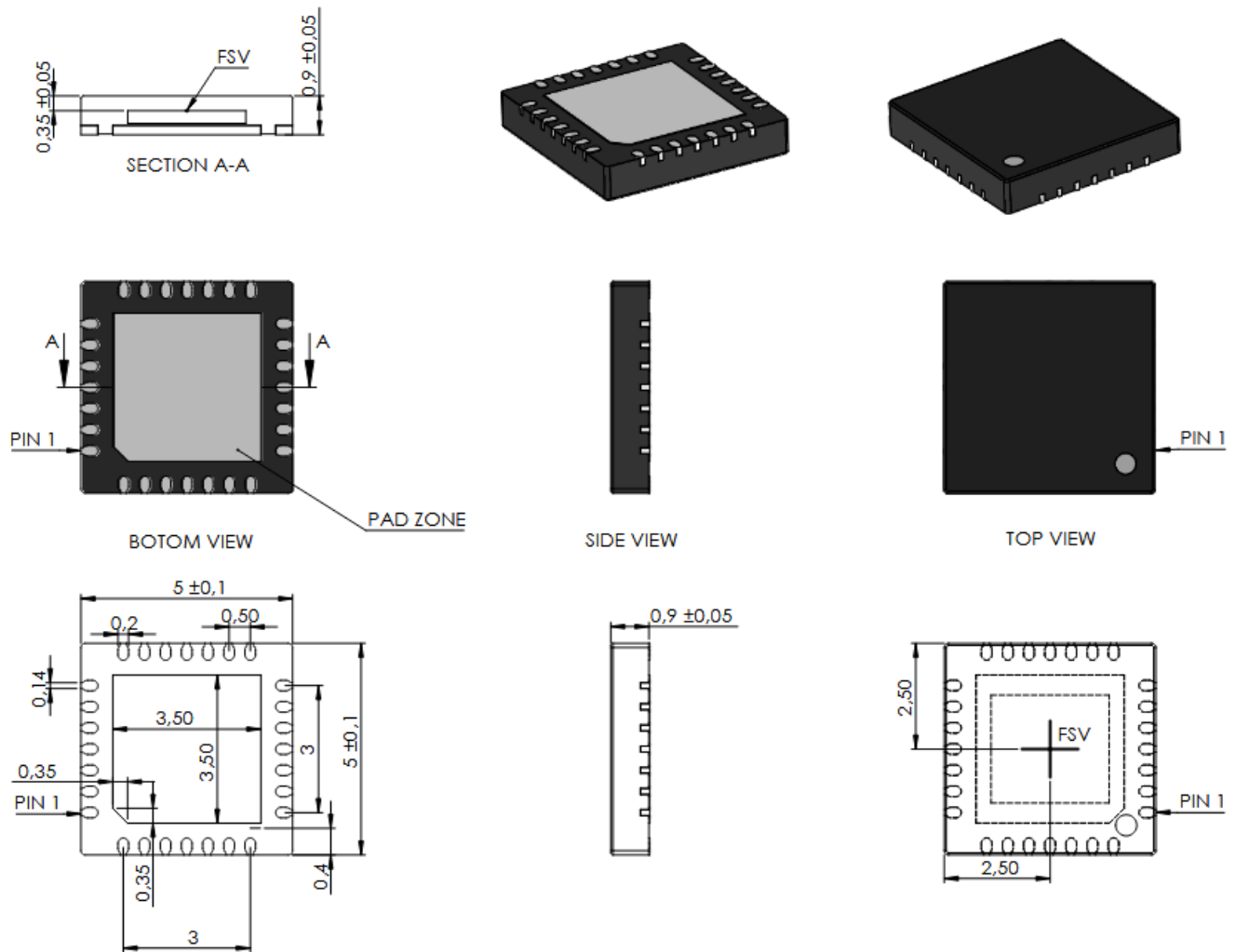
Figure 1: Dimensions of QFN 5x5 mm 2 package with 28 pads. All dimensions are in units mm. The field sensitive volume (FSV) is located at the center of the package. Not to scale.
